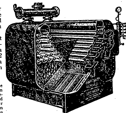
Tubular-Spencer Steam Heater
