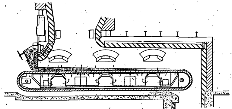
FIG. 8. OVERFEED TRAVELING-GRADE STOKER
