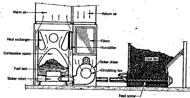
FIG. 4. STOKER-FIRED WINTER AIR CONDITIONING UNIT
