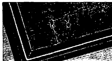
Above close-up of Mundet Natural Cork Isolation Mat shows how the blocks of cork are held together within a rigid steel frame.
