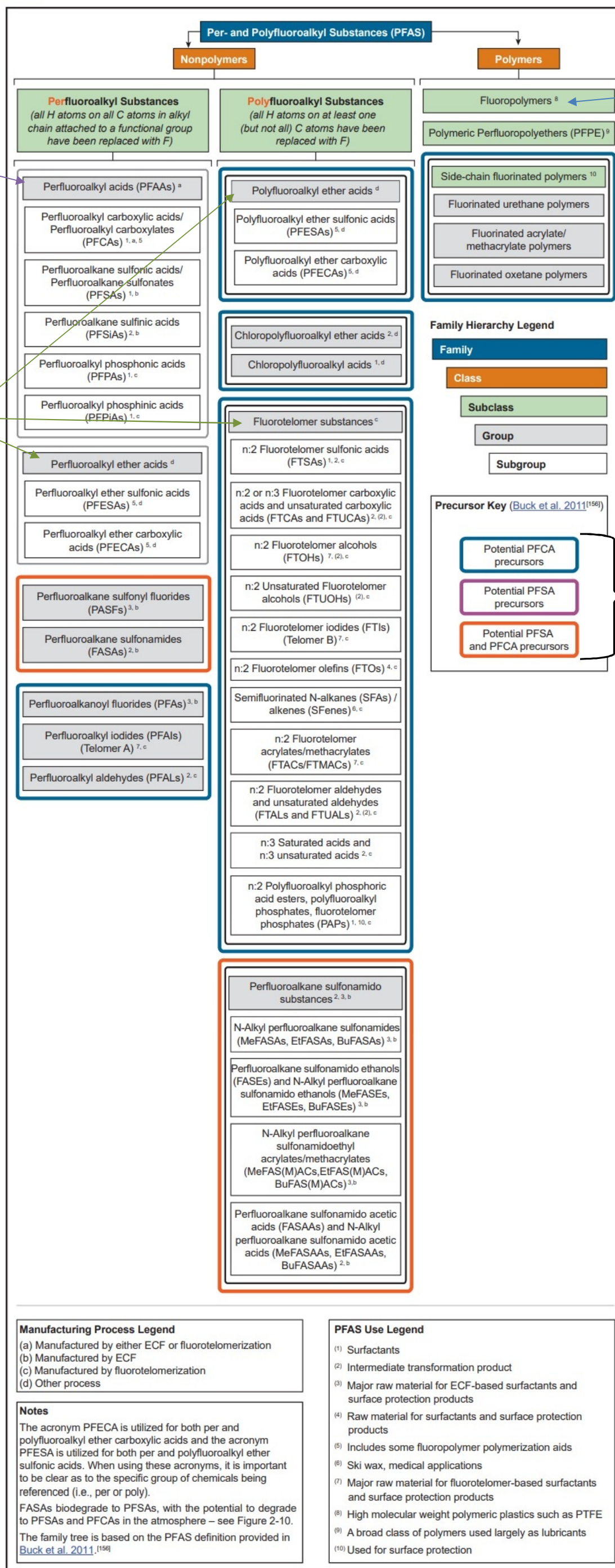
Fig.3 PFAS family tree
