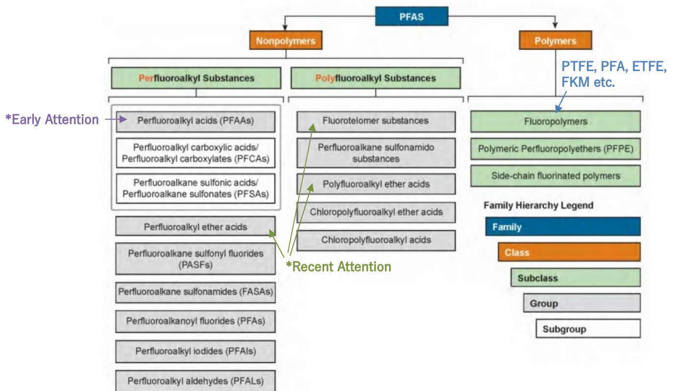
Fig. 2 The PFAS family
