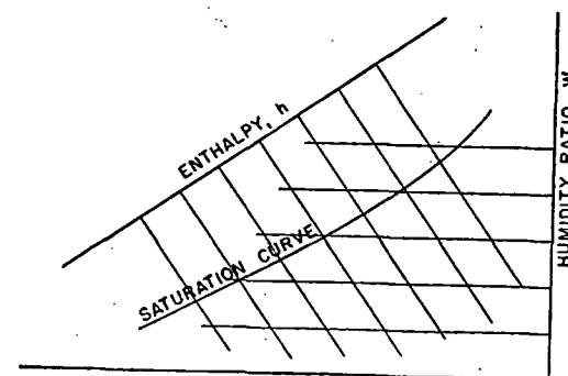
FIG. 3. BASIC COORDINATES OF A.S.H.A.E. PSYCHROMETRIC CHART
