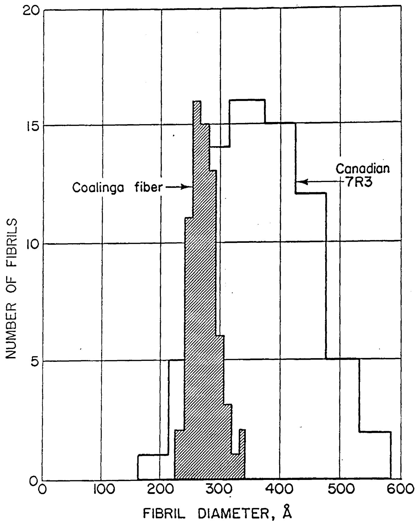
FIG. 6 : Histogram of fibril diameter distribution.
