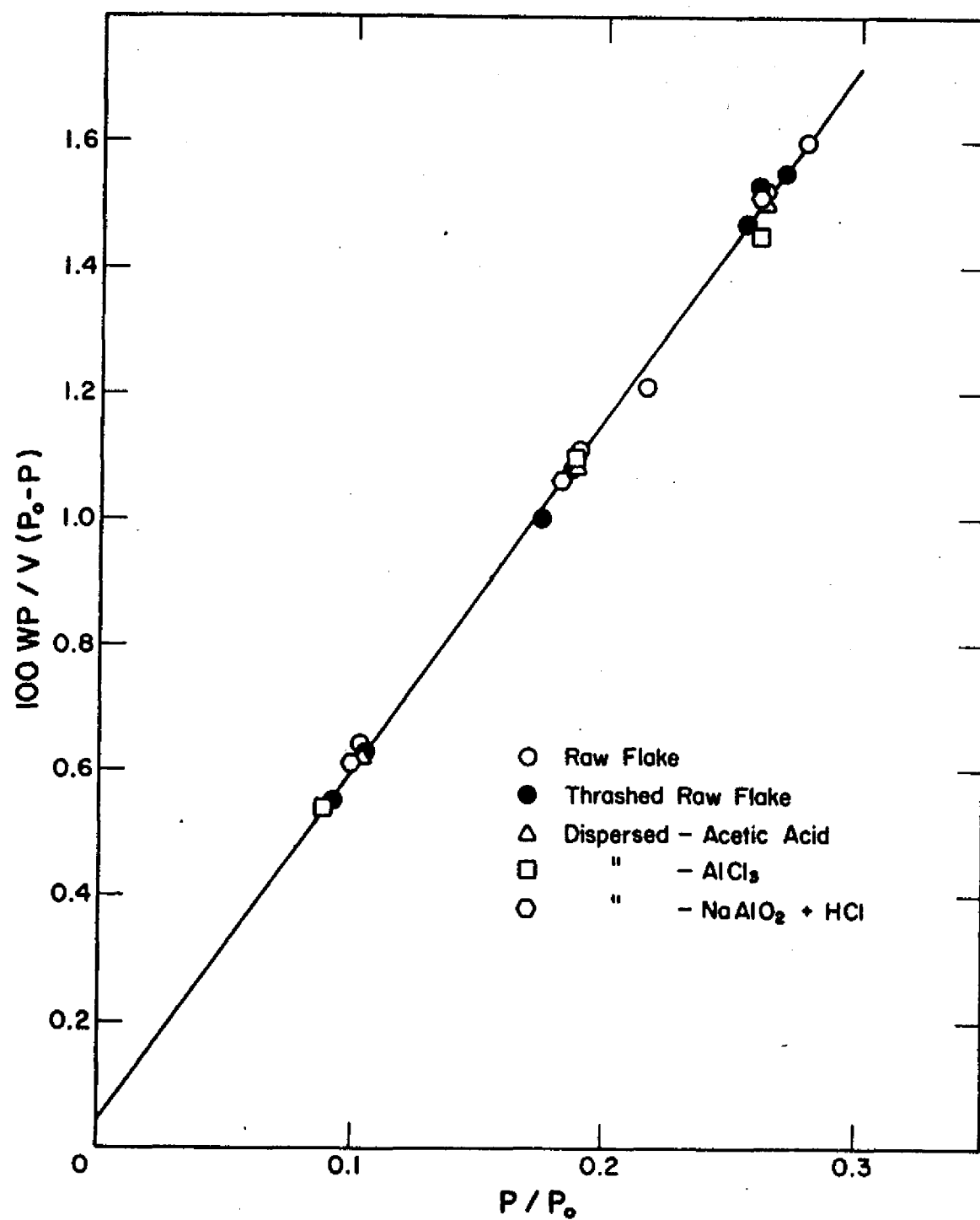
FIG. 5: BET plot for Coalinga flake chrysotile.
