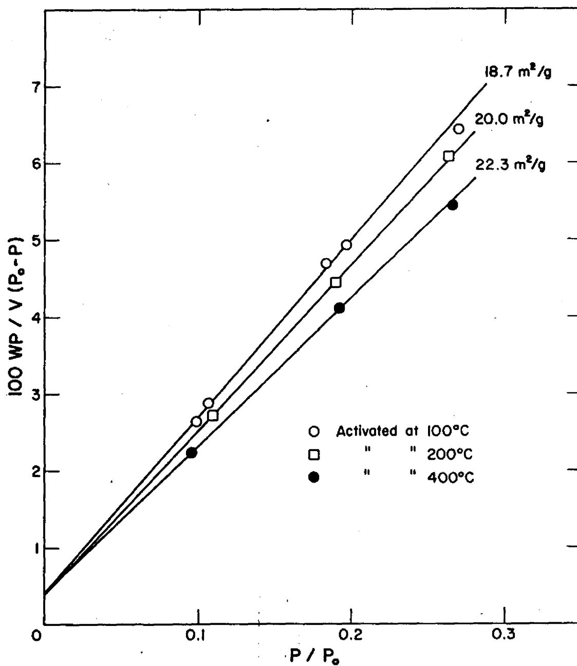
FIG. 4: BET plot for Cassiar chrysotile.
