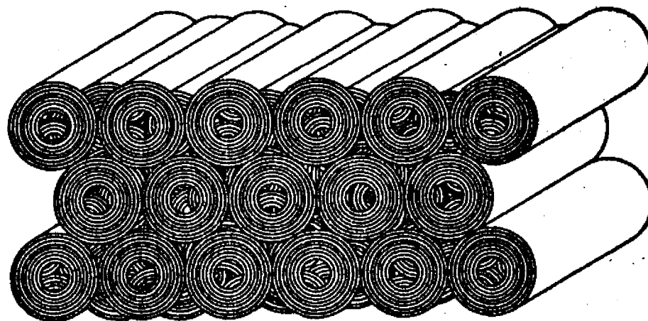
b. Idealized closed structure (after Whittaker)
