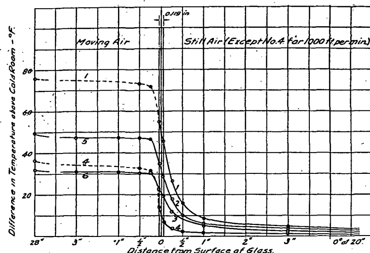
FIG. 2. TEMPERATURE GRADIENT CURVES FOR GLASS (TAKEN FROM BULLETIN No. 24, ENGRG. EXP. STA., PENNA. STATE COLLEGE)
