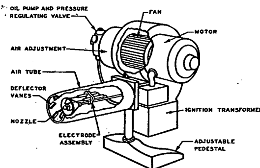
FIG. 12. HIGH-PRESSURE ATOMIZING OIL BURNER
