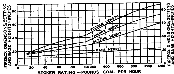
FIG. 11. SUGGESTED MINIMUM FIREBOX DIMENSIONS AND BASE HEIGHTS 2
