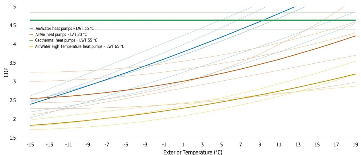
Figure 43. COPfText curves
