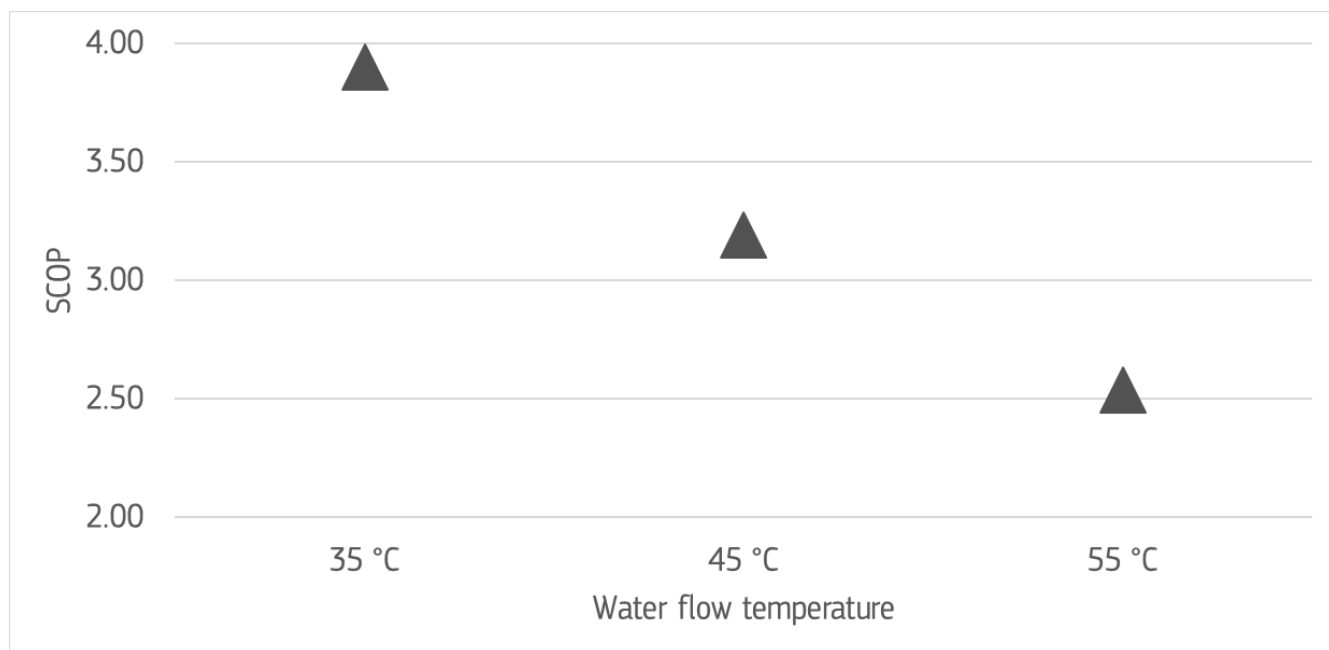
Figure 47. Comparison of the Seasonal Performance Factor for different water flow temperatures
