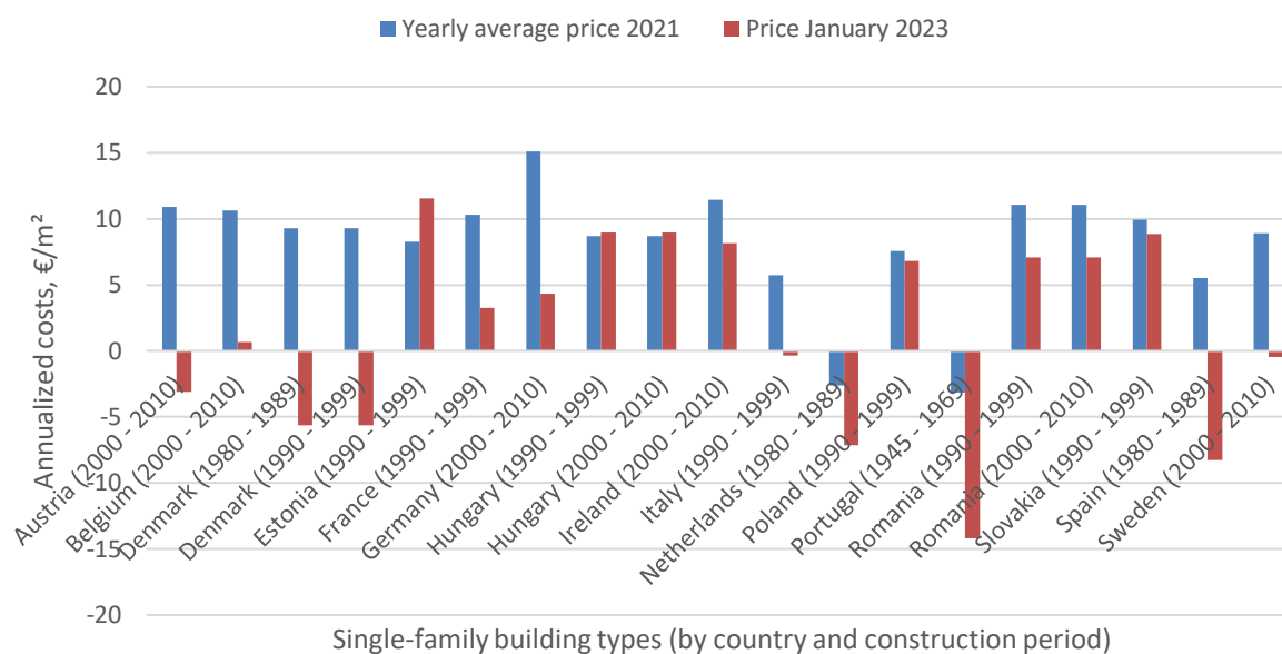
Figure 51. Total early average costs from switching from gas to heat pump (including savings on energy and investment cost)
