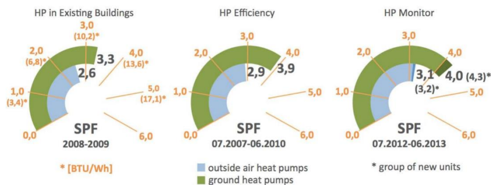
Figure 48. SPF for different houses
