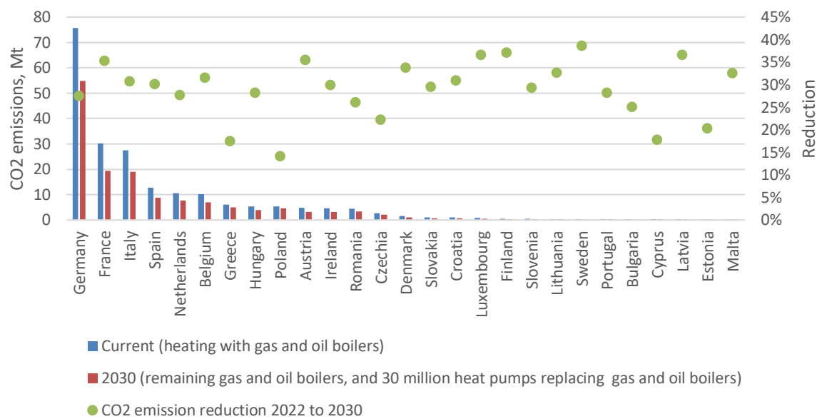
Figure 20. CO 2 emissions from heating residential households with gas and oil boilers in 2022 and 2023 in 27 EU countries (Scenario 1)
