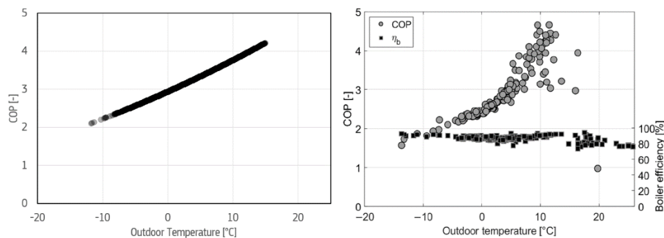
Figure 46. Air/Water heat pump performance curve from the current study (left) and Air/Water heat pump performance curve from Neubert et al, 2022 (right)
