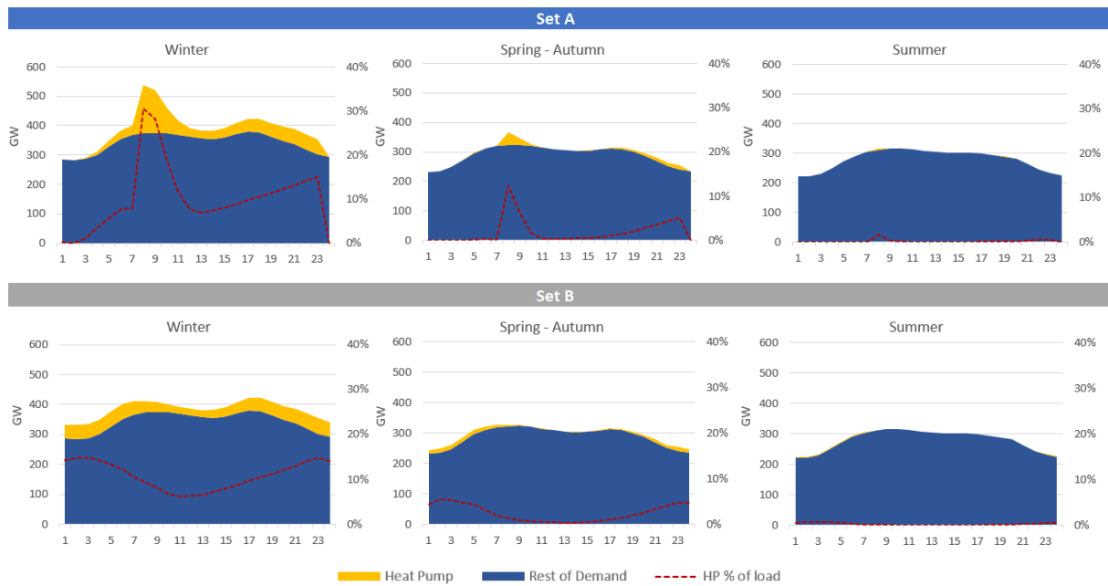
Figure 23. EU average seasonal hourly electricity demand profiles in Scenario 1 for Set A and B (hourly total and heat pump % share of total grid demand)
