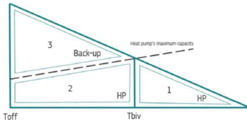
Figure 44. System states of a hybrid heat pump
