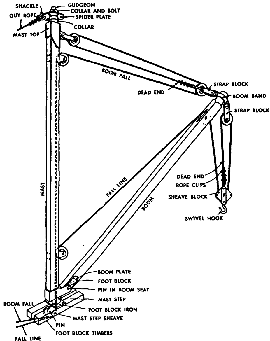
FIG 25-15 —Diagram of guy derrick (For simplicity, only one guy is shown )
