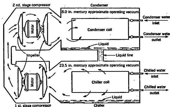
FIG. 9. ENCLOSED TYPE CENTRIFUGAL CONDENSING UNIT
