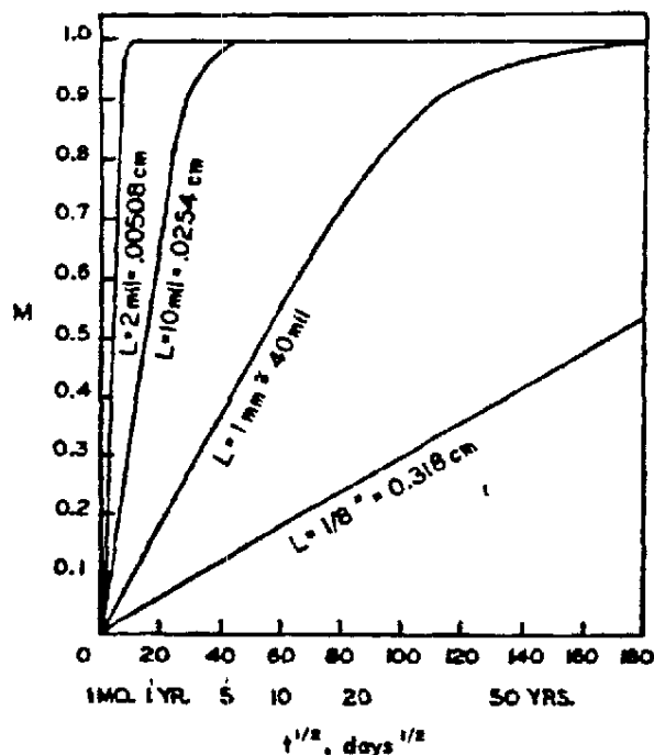
Fig. 1. Fraction of initial VCM content lost ( M ) vs square root of
