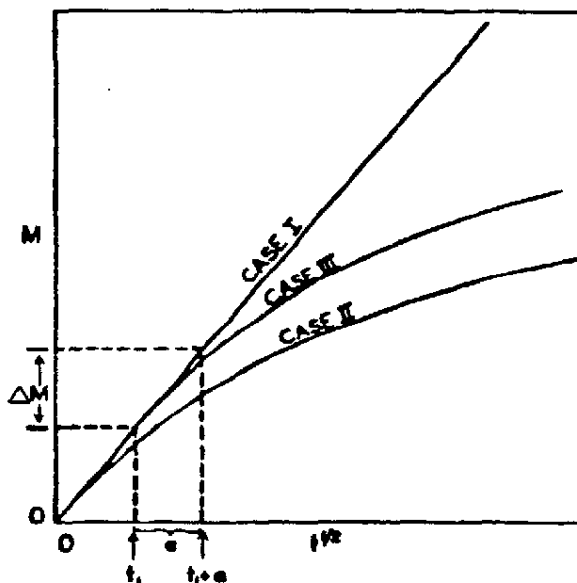
Fig. 6. Schematic comparison of fractional VCM loss ( M ) vs t^{1/2} curves for Cases I, II, and III.
