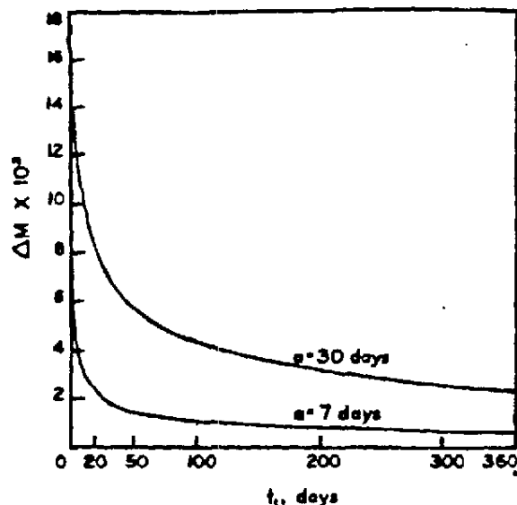
Fig. 7. Fraction of original VCM content entering pipe contents ( \Delta M ) for 7 and 30-day extraction periods vs pipe age at start of extraction ( t_1 ), calculated for \frac{1}{2} in. wall thickness and 30^\circ\text{C} . Case III.
