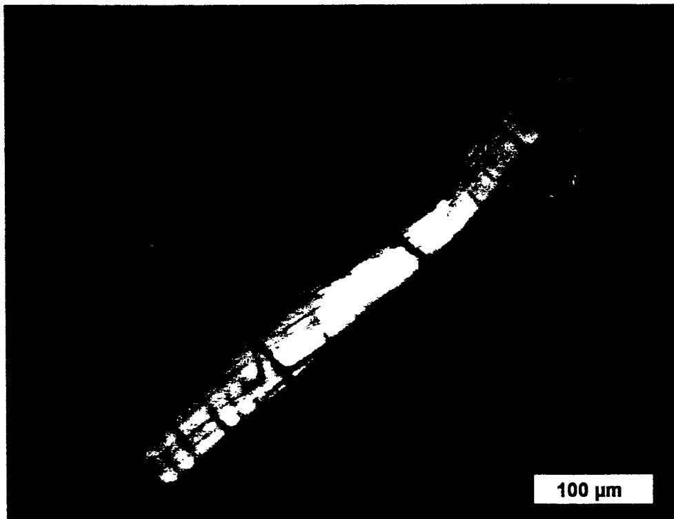
Figure 4. Chrysotile fiber bundle, partially crossed polars.
