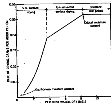
FIG. 5. RATE OF DRYING OF WHITING SLAB
