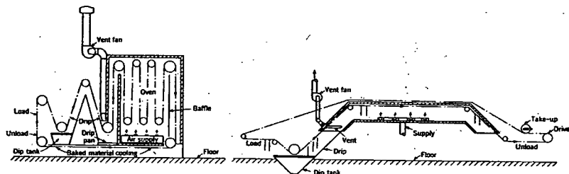
FIG. 3. SMALL PART MULTIPLE PASS OVEN FIG. 4. INCLINED END ENAMELING OVEN
