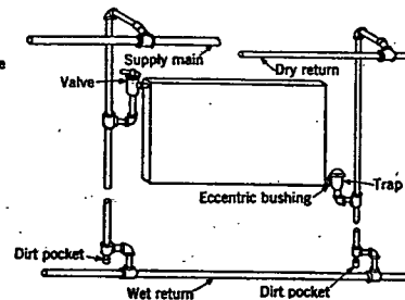
FIG. 46. TWO-PIPE CONNECTIONS TO RADIATOR HUNG ON WALL
