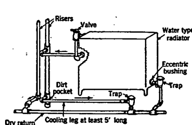
FIG. 45. TWO-PIPE TOP AND BOTTOM OPPOSITE END RADIATOR CONNECTIONS
