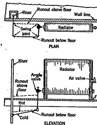
FIG. 44. ONE-PIPE RADIATOR CONNECTIONS
