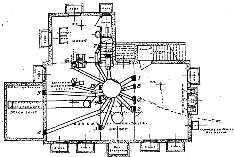
FIG. 9. BASEMENT PLAN
