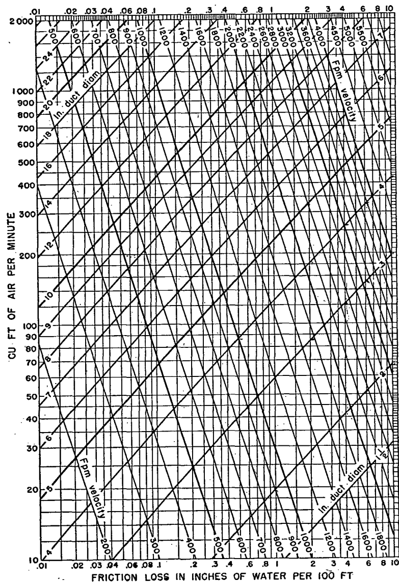
FIG. 1. FRICION OF AIR IN STRAIGHT DUCTS
