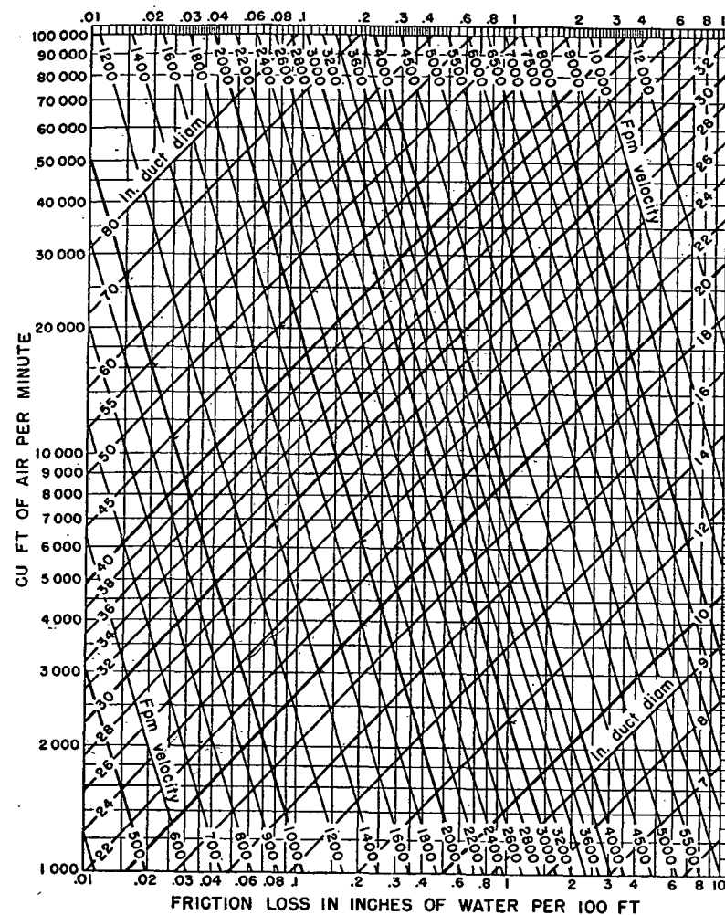
FIG. 2. FRICION OF AIR IN STRAIGHT DUCTS
