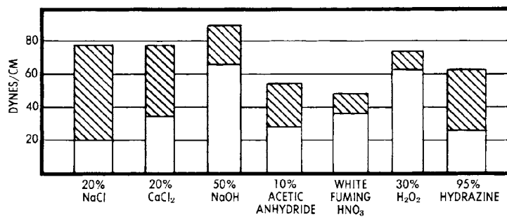
FIG. 45. Surface activity of \text{C}_8\text{F}_{17}\text{SO}_3\text{K} in various chemical media. The tops of the columns represent surface tension without surfactant added. The shaded areas indicate the surface tension reductions obtained with \text{C}_8\text{F}_{17}\text{SO}_3\text{K} .
