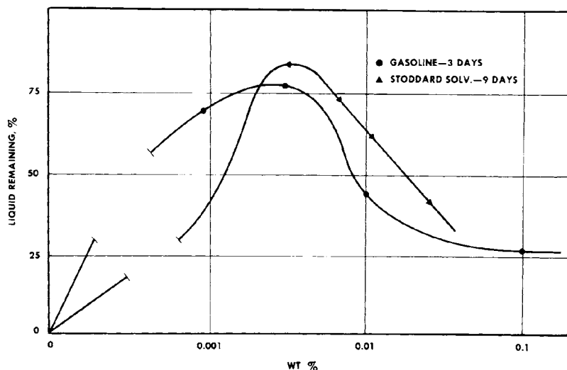
FIG. 52. Effect of concentration of surfactant F-2 on inhibiting action of rate of evaporation.
