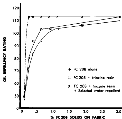
FIG. 70. The effect of a triazine resin and a hydrocarbon water repellent on oil repellency of a cotton fabric treated with a commercial fluorocarbon resin FC-208.
