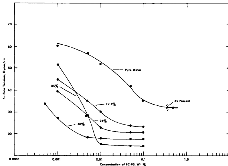
FIG. 40. Surface activity of \text{C}_8\text{F}_{17}\text{SO}_3\text{K} in aqueous phosphoric acid.
