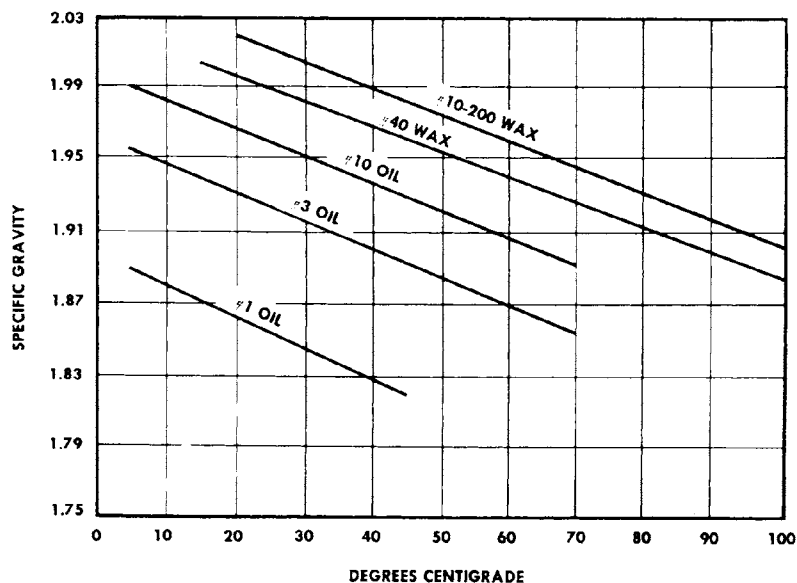
FIG. 28. Specific gravity of chlorofluorocarbon oils and waxes.
