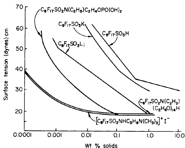
Fig. 36. Surface activity of various fluorocarbon sulfonic acid derivatives in water.
