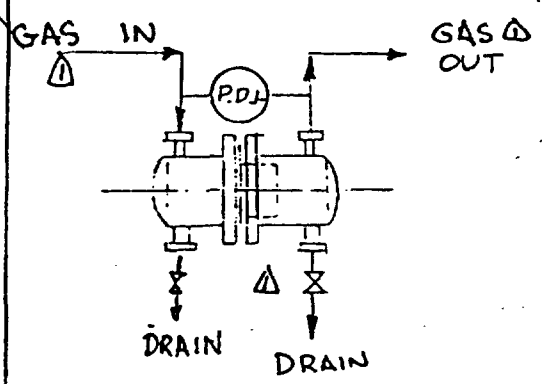
PIPING SCHEMATIC
