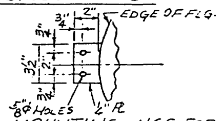
MOUNTING LUGS FOR SIZES 10" TO 14"
