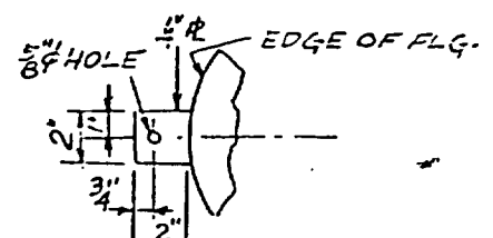
MOUNTING LUGS FOR SIZES 4" TO 8"
