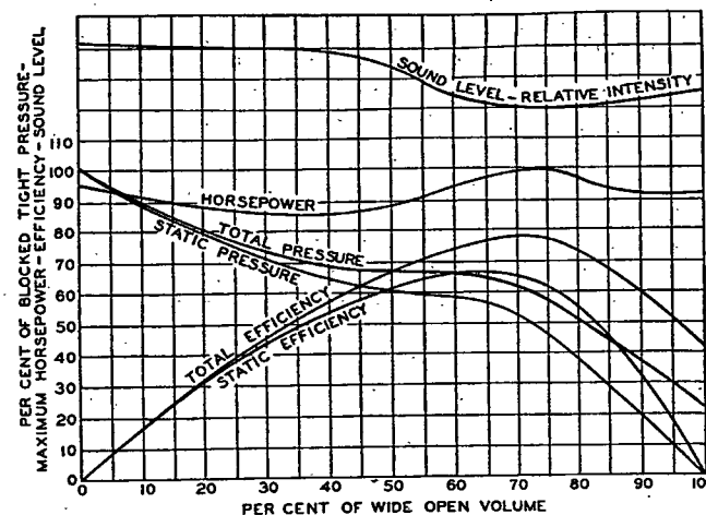
FIG. 1. OPERATING CHARACTERISTICS OF AXIAL FLOW AIRFOIL TYPE FAN
