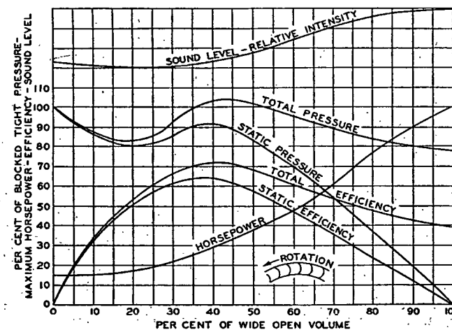
FIG. 2. OPERATING CHARACTERISTICS OF A FAN WITH BLADES CURVED FORWARD
