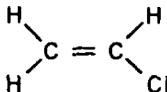
Vinyl Chloride
