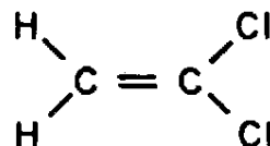
Vinylidene Chloride
