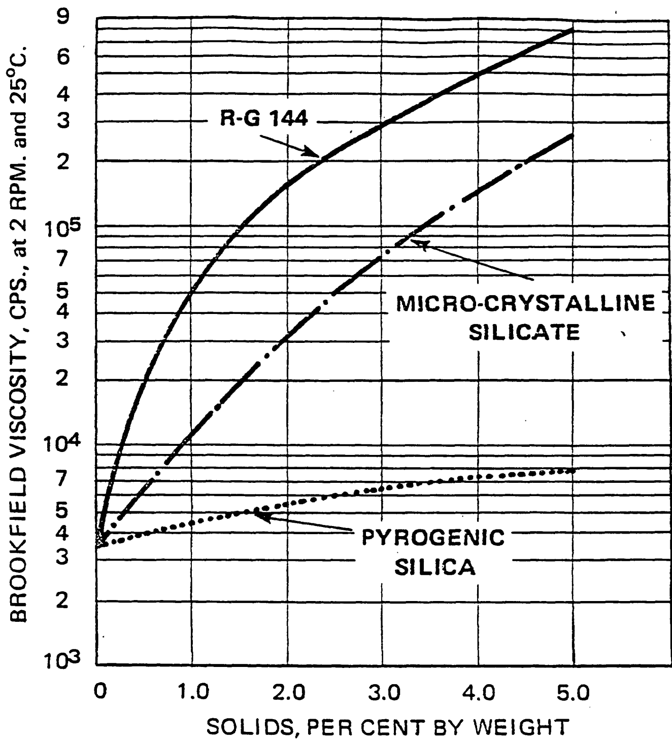
EFFECT ON VISCOSITY OF VARIOUS THICKENERS IN BAKELITE RESIN HARDENER ZZL-0814
