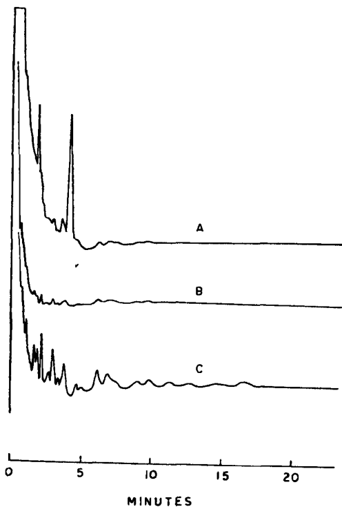
Fig. 1: Chromatograms of foam plug blanks, OV-17/QF-1
