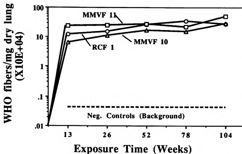
Figure 1. Lung burdens, expressed in WHO fibers/mg dry lung tissue, in rats exposed continuously to 30 \text{ mg/m}^3 of RCF 1, MMVF 10, or MMVF 11. A WHO fiber is defined as having length:diameter ratio of \geq 3 , a diameter < 3 \mu\text{m} and a length \geq 5 \mu\text{m} .
