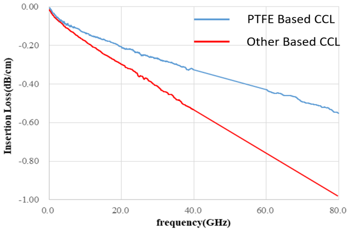
Fig 2. Transmission Loss of PTFE CCL and Other CCL
