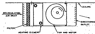
Fig. 9....Suspended Centrifugal Unit Heater—Cabinet Type
