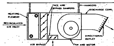
Fig. 10....Suspended Centrifugal Unit Heater—Industrial Type—Bypass Controlled
