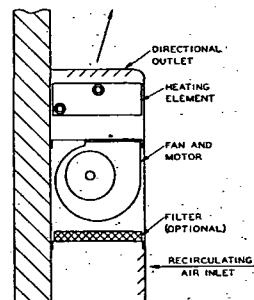
Fig. 8....Floor-Mounted Centrifugal Unit Heater—Cabinet Type
