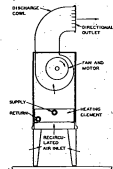
Fig. 11....Floor-Mounted Centrifugal Unit Heater—Industrial Type—Valve Controlled
