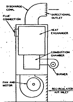
Fig. 13....Oil-Fired Centrifugal Fan Unit Heater—Floor Mounted
