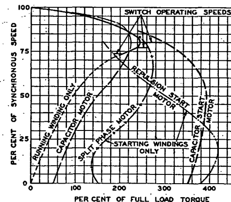
FIG. 10. SPEED-TORQUE CHARACTERISTICS OF SINGLE PHASE MOTORS.
