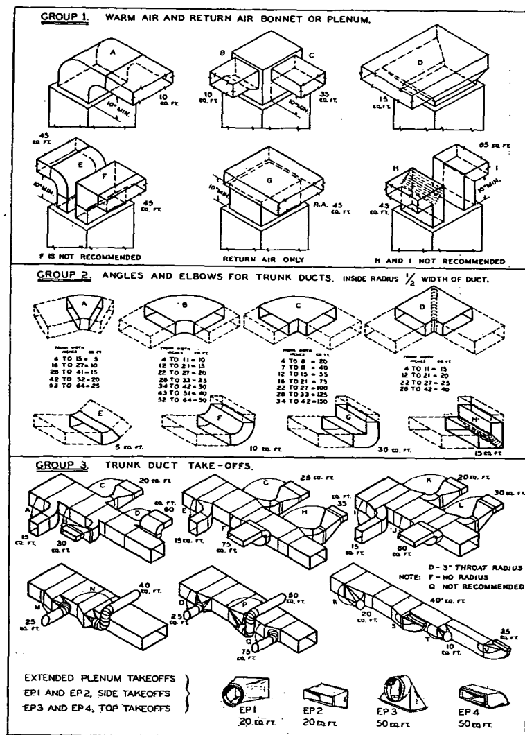
Fig. 7.... Equivalent Length of Fittings and Intakes
