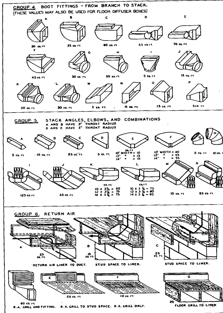
Fig. 7.... Equivalent Length of Fittings and Intakes (Concluded)
