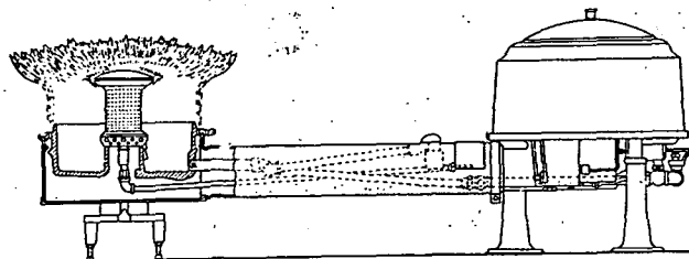
FIG. 13. POT TYPE VAPORIZING BURNER
