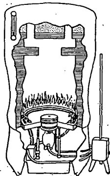
FIG. 12. WALL FLAME VERTICAL ROTARY BURNER
