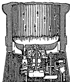
FIG. 11. CENTER FLAME VERTICAL ROTARY BURNER
