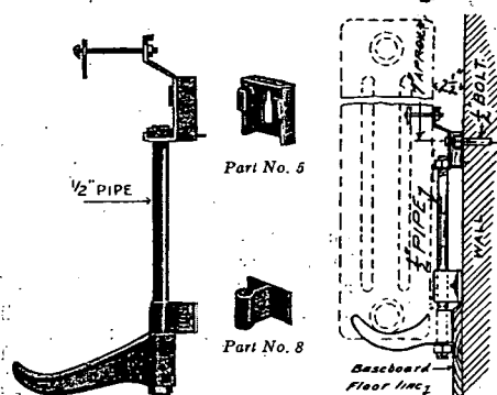
Style "H" Hanger, with baseboard adjustment
