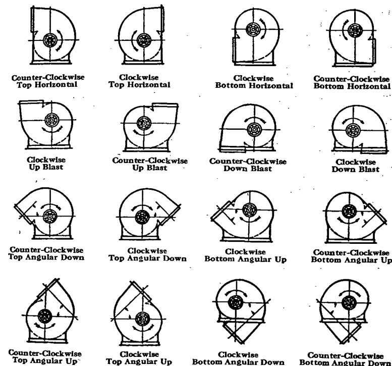
FIG. 7. DESIGNATION OF DIRECTION OF ROTATION AND DISCHARGE
