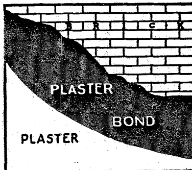
PLASTER BOND METHOD.
