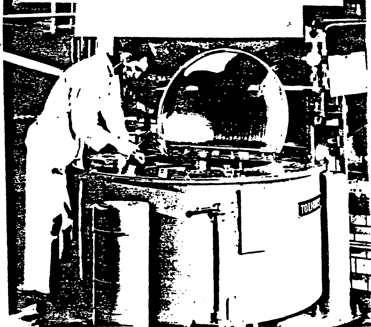
Figure 11 Top Unloading 48" Tolhurst Centrifuge Monsanto Company Nitro, West Virginia
