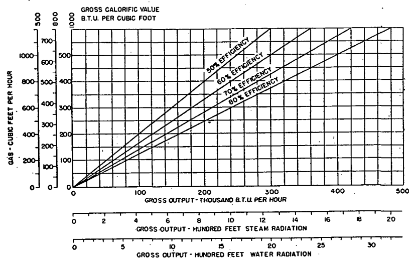
FIG. 3. GAS FUEL BURNING RATE CHART
