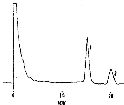
FIG. 1.—Electron capture GLC curve from the 0.2 ml \text{SbCl}_3 (Hooker Chemical) perchlorination of 0.50 \mu g Aroclor 1221; 0.51 ng equivalent Aroclor 1221 injected. Peak 1 represents 0.81 ng DCB. Peak 2 represents 0.28 ng BNCB.
