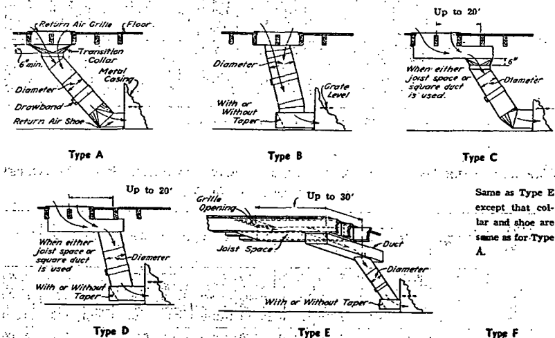
FIG. 5. TYPICAL ARRANGEMENTS OF RETURN AIR DUCT SYSTEMS
