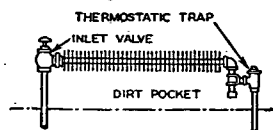
FIG. 48. TYPICAL CONNECTIONS TO FINNED PIPE CONVECTOR
