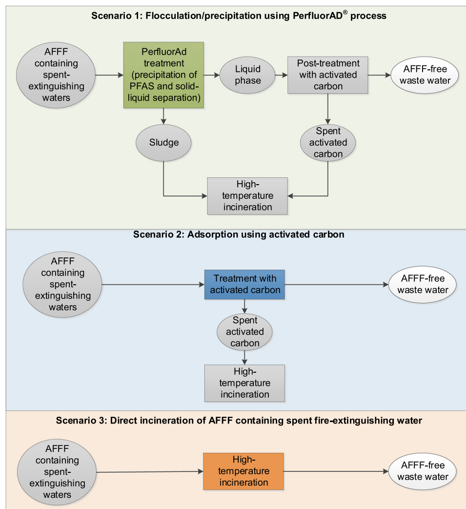
FIGURE 3 Scenarios for treating aqueous film-forming foams (AFFFs) containing spent fire-extinguishing waters using functional precipitation agents (scenario 1), activated coal (scenario 2), and direct incineration (scenario 3). PFAS = per- and polyfluoroalkyl substances.
