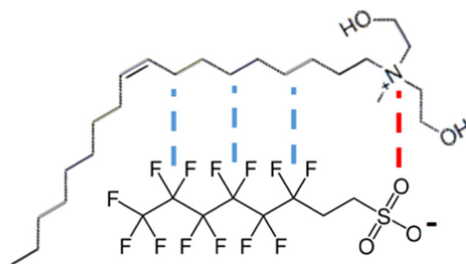
FIGURE 2: Schematic example representing the binding interactions of one 1H,1H,2H,2H perfluorooctanesulfonate ( \text{H}_4\text{PFOS} ) anion with the Bis(hydroxyethyl)methylethylammonium cation in aqueous solution.
