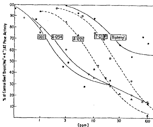
FIG. 2. Concentration dependence of brain ( \text{Na}^+ + \text{K}^+ )-ATPase inhibition by DDT, Aroclor 1254, Aroclor 1221, 2-chlorobiphenyl and biphenyl. Ten microliters of a dimethyl sulfoxide solution of each chlorinated hydrocarbon were added 3 sec after addition of 40 \mu\text{g} of enzyme protein to initiate the ATPase assay.
