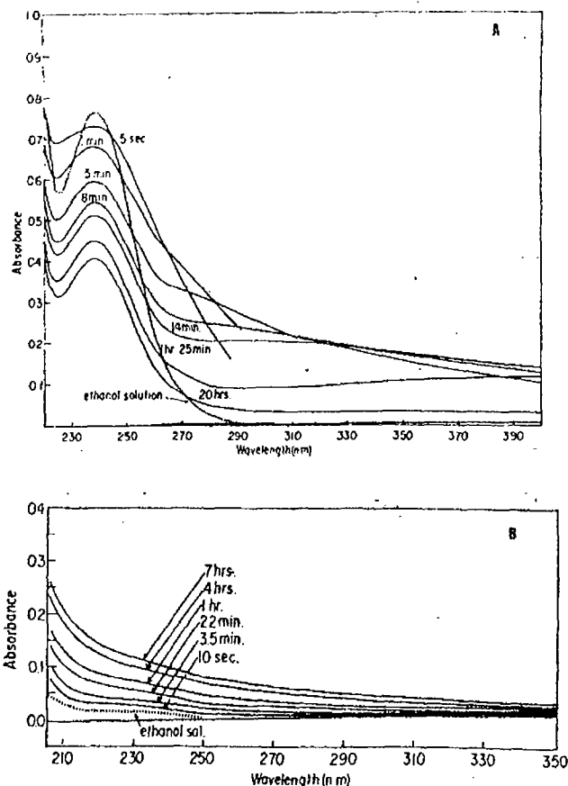
FIG. 1. Absorption spectra of 67 \mu\text{M} 2-chlorobiphenyl (A) and 25 \mu\text{M} Tris-oleate (B) in ethanol (—) and in 1% ethanol in water (---). Spectral alterations in the ethanol-water solutions were determined at the indicated intervals after preparation. Spectra were recorded with a Beckman Acta V spectrophotometer.
