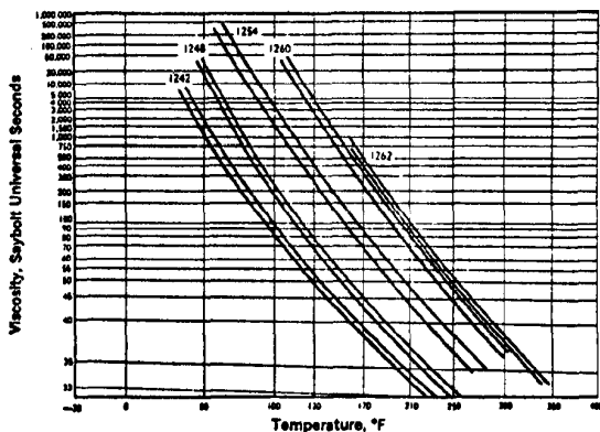
Fig. 3 — Viscosity Ranges of Some Aroclor® Plasticizers
