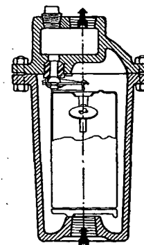
No. 811-816, Blast Type
