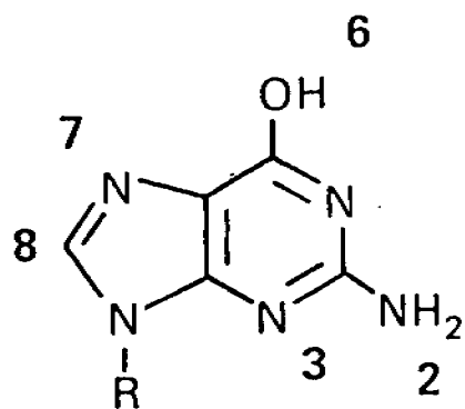
Guanine
