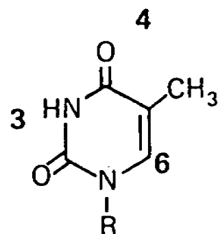
Thymine
