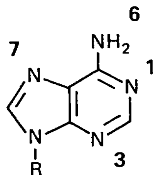
Adenine
