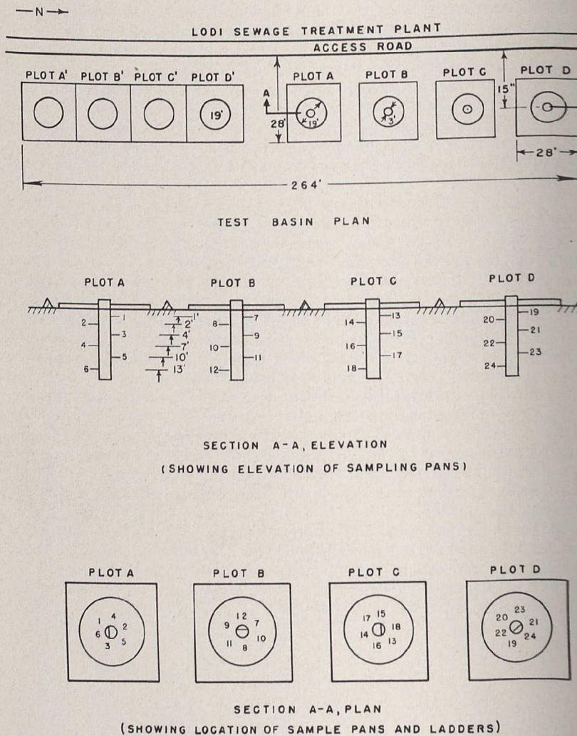
FIGURE 15. Spreading basin layout, Lodi, California
