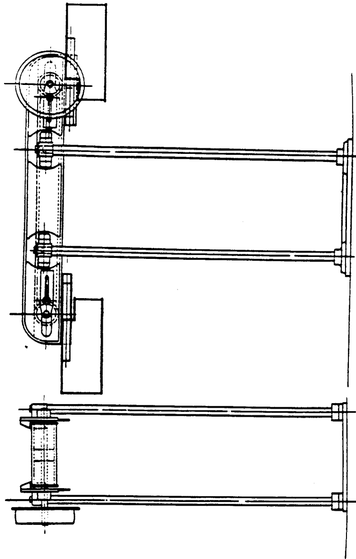
FIG. 3.—REVERSIBLE BIDDING LATTICE.
