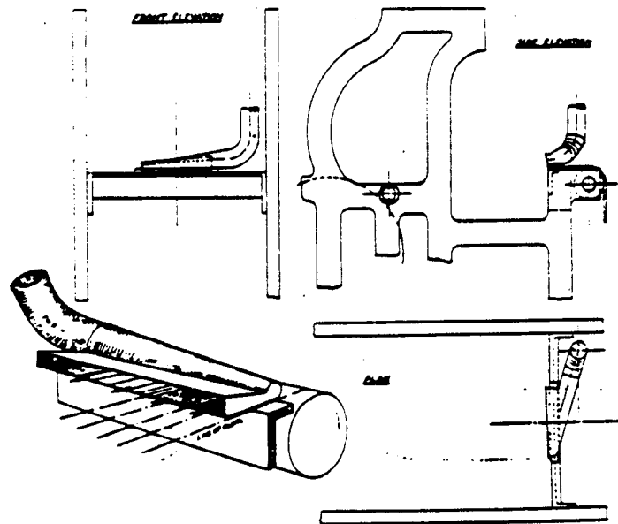
FIG. 15.—EXHAUST VENTILATION AT BRAKE BAND LINTING LOOM. Applied at Breast.
