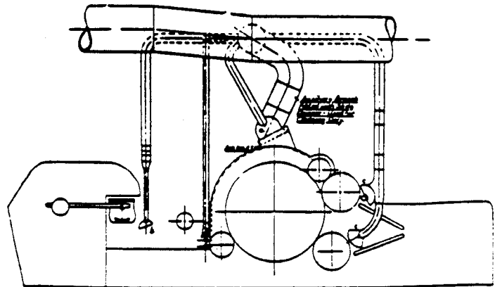
FIG. 6.—EXHAUST FOR CARDING MACHINES.
