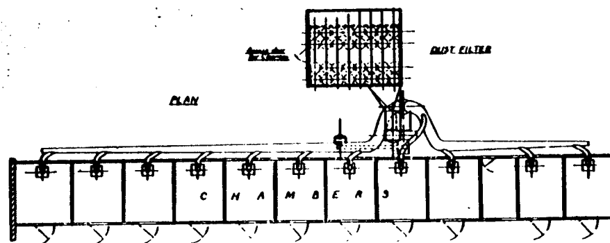
FIG. 4.—EXHAUST AT DISINTEGRATOR CHAMBERS. Disintegrators (not shown) are above the chambers.
