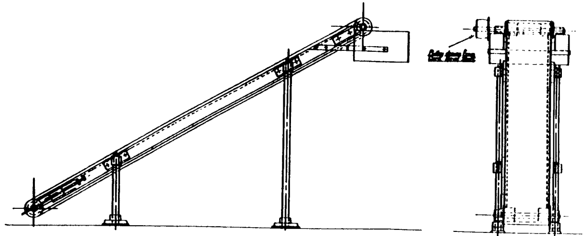
FIG. 8.—LATTICE FOR COLLECTION OF CARDED FIBRE.
