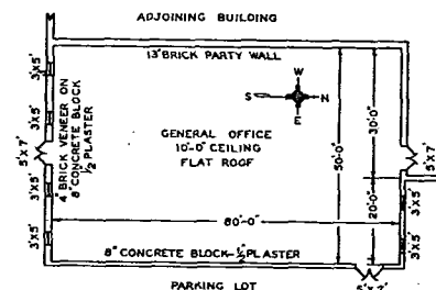
Fig. 6—Plan of One-Story Office Building
