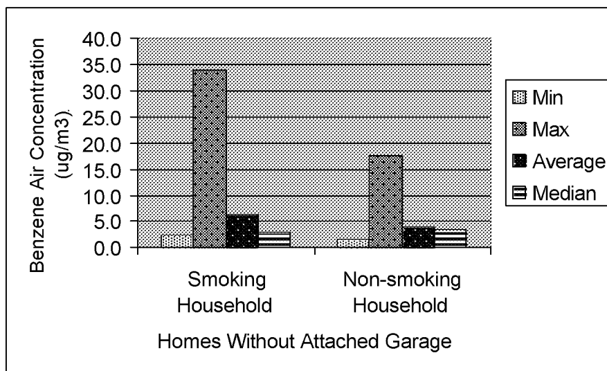
Figure 7.5: Comparison of Indoor Air Concentrations of Benzene in Smoking and Non-Smoking Households
