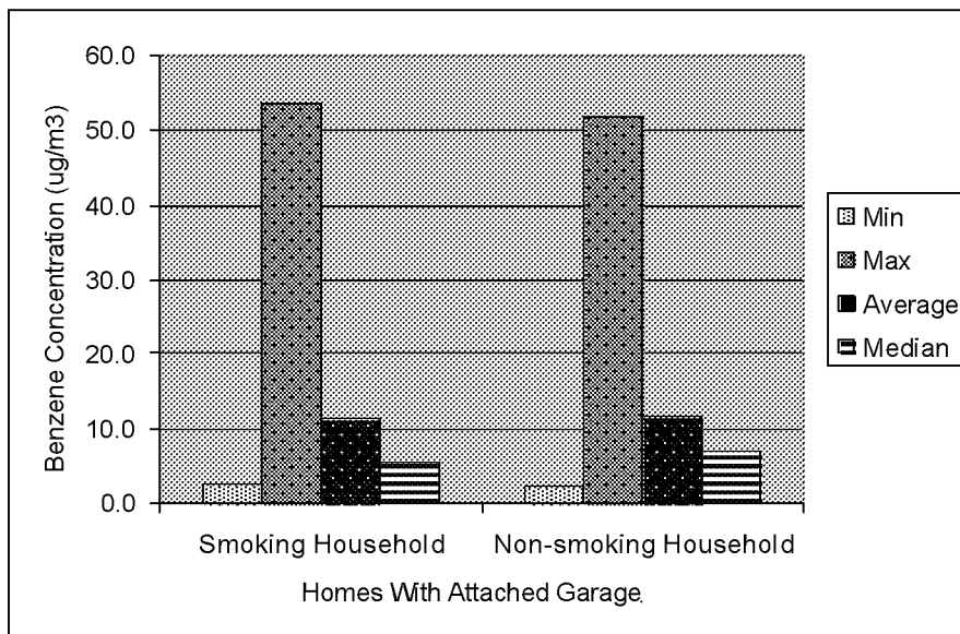
Figure 7.2 Comparison of Indoor Air Benzene Concentrations in Smoking and Non-Smoking Households with Attached Garages
