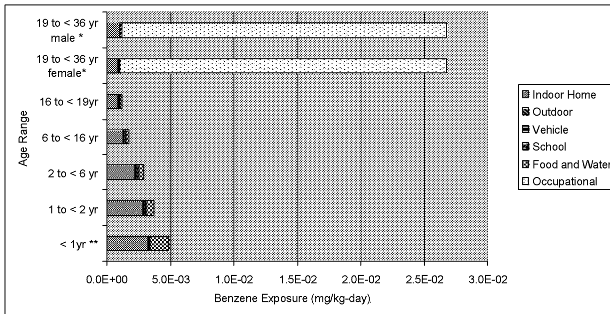
Figure 7.7 Contribution of Various Ambient Sources to Benzene Exposures High-end Total Background
