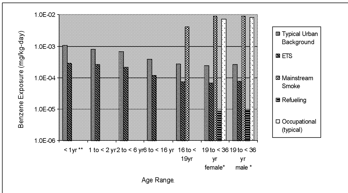
Figure 7.8 : Comparison of Benzene Exposures from Typical Urban Background (Ambient) Sources to Specific Sources
