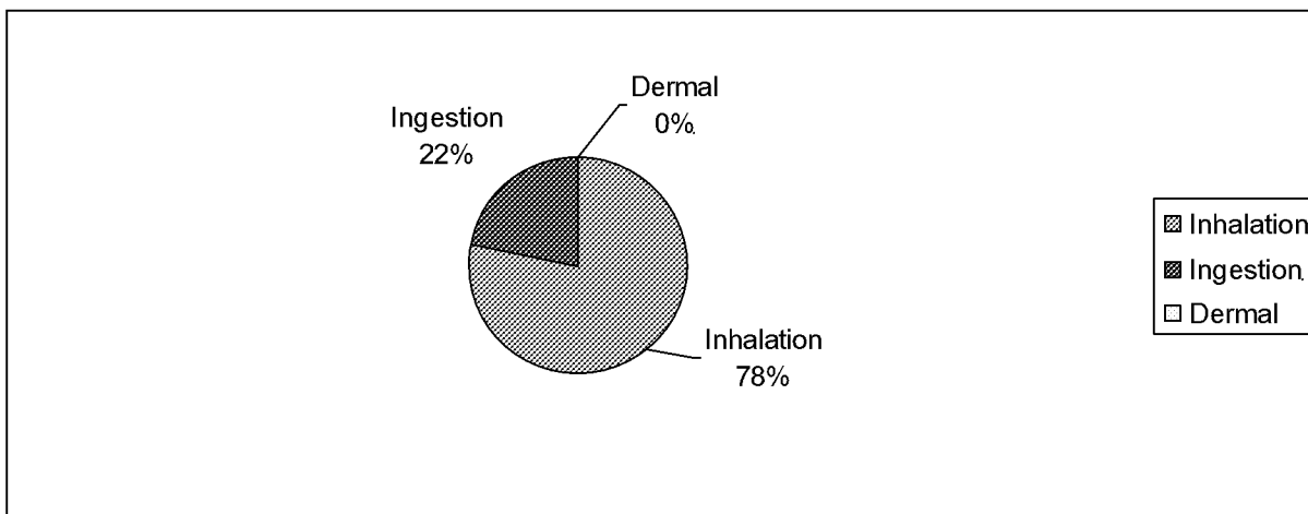
Figure 7.4 Predominant Pathways of Benzene Exposure for Nursing Infants (with occupationally exposed mothers) from Ambient Sources
