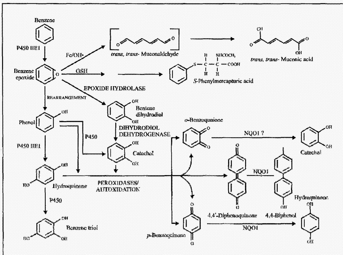
Figure 1. Major metabolic pathways in benzene toxicity.
