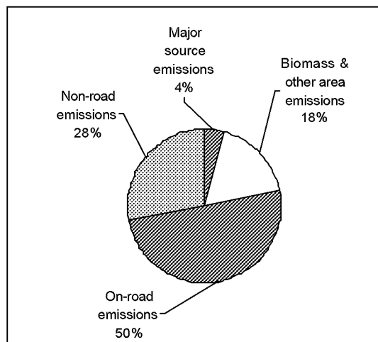
Figure 5.1: Relative Contribution of Various Benzene Emission Sources to Total Benzene Emissions from 1996 NTI database
