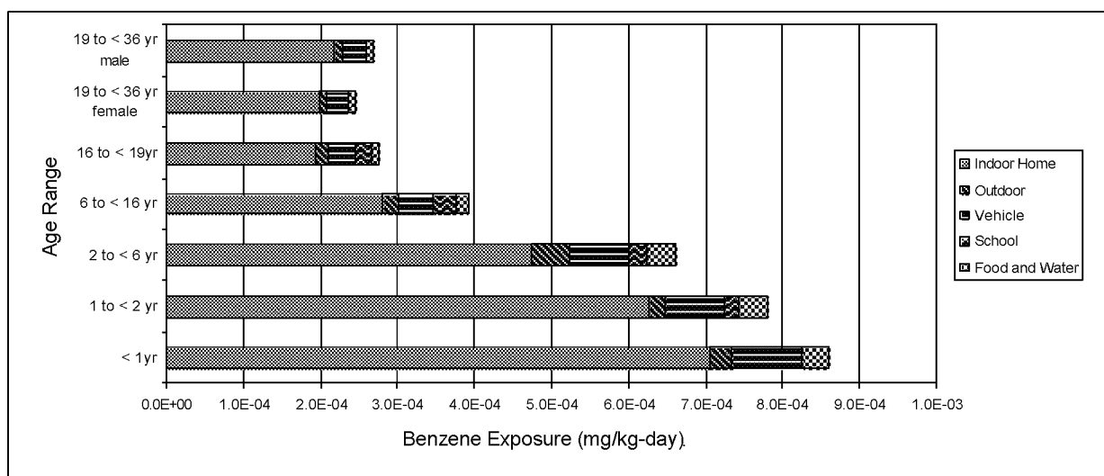
Figure 7.6: Contribution of Various Ambient Sources to Typical Total Background Benzene Exposures
