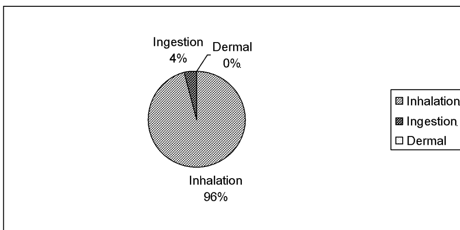
Figure 7.3. Predominant Pathways of Benzene Exposure for Children and Prospective Parents from Ambient Sources
