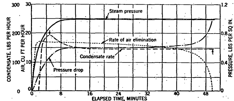
FIG. 18. RELATION BETWEEN ELAPSED TIME, STEAM PRESSURE, CONDENSATE AND AIR ELIMINATION RATES
