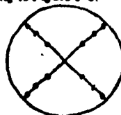
Figure 3-4. Cross section of circular stack showing location of traverse points on perpendicular diameters.
