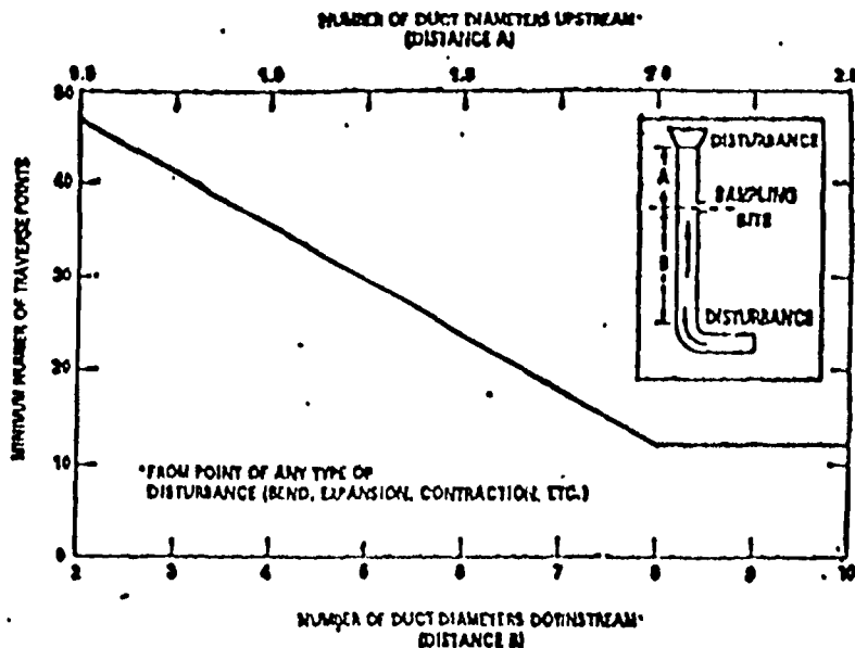
Figure 1-3. Minimum number of traverse points.
