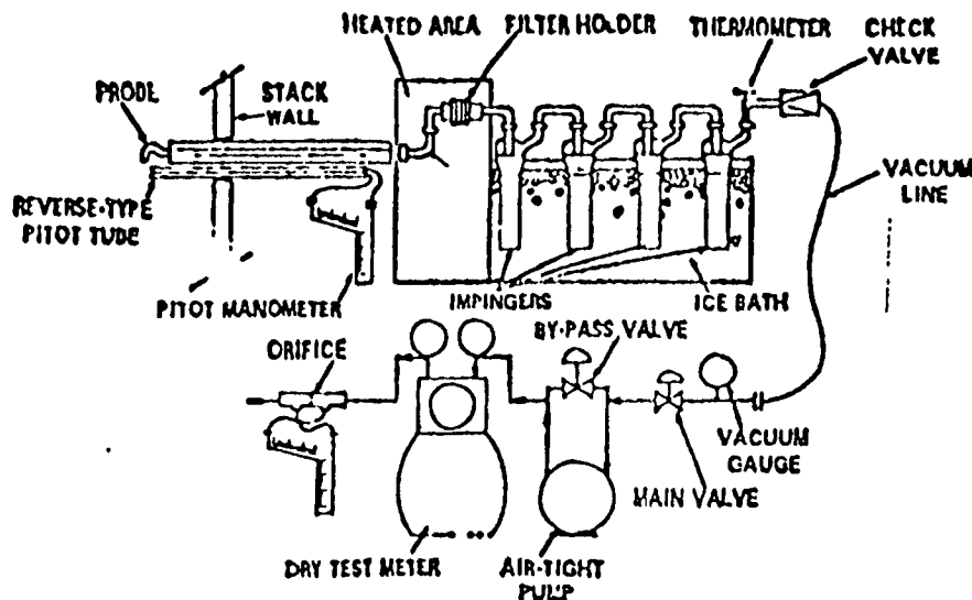
Figure 3-1. Particulate-sampling train.
