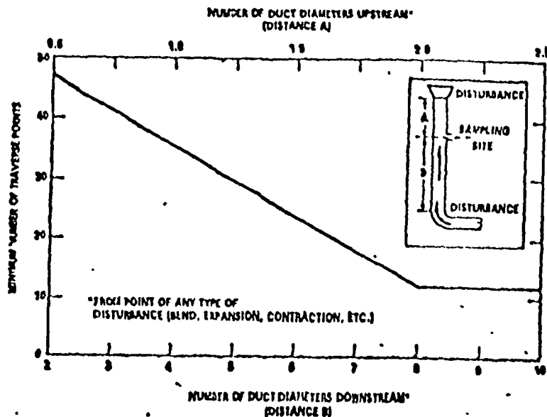
Figure 3-3. Minimum number of traverse points.
