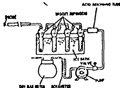
FIGURE 2-1. Sampling train.
