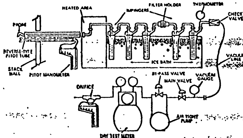
Figure 1-1. Particulate-sampling train
