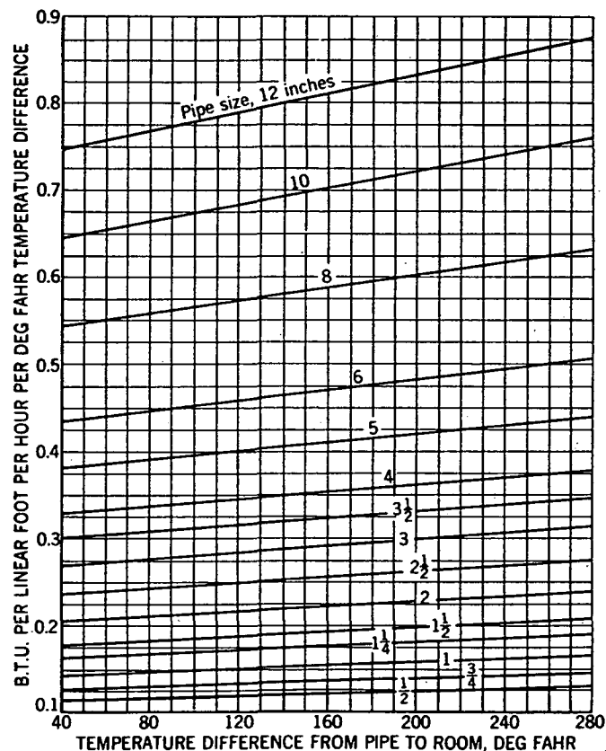
FIG. 3. HEAT LOSS THROUGH 1½ IN. THICK 85 PER CENT MAGNESIA TYPE COVERING
