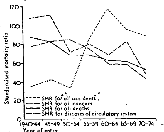
Fig. 2 Standardised mortality ratios for all deaths, all cancers, diseases of circulatory system, and accidents related to the year of entry into industry.
